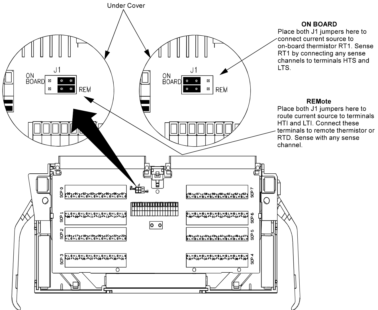
Figure 2-8 Temperature Sensing for HP E1419 Terminal Module
