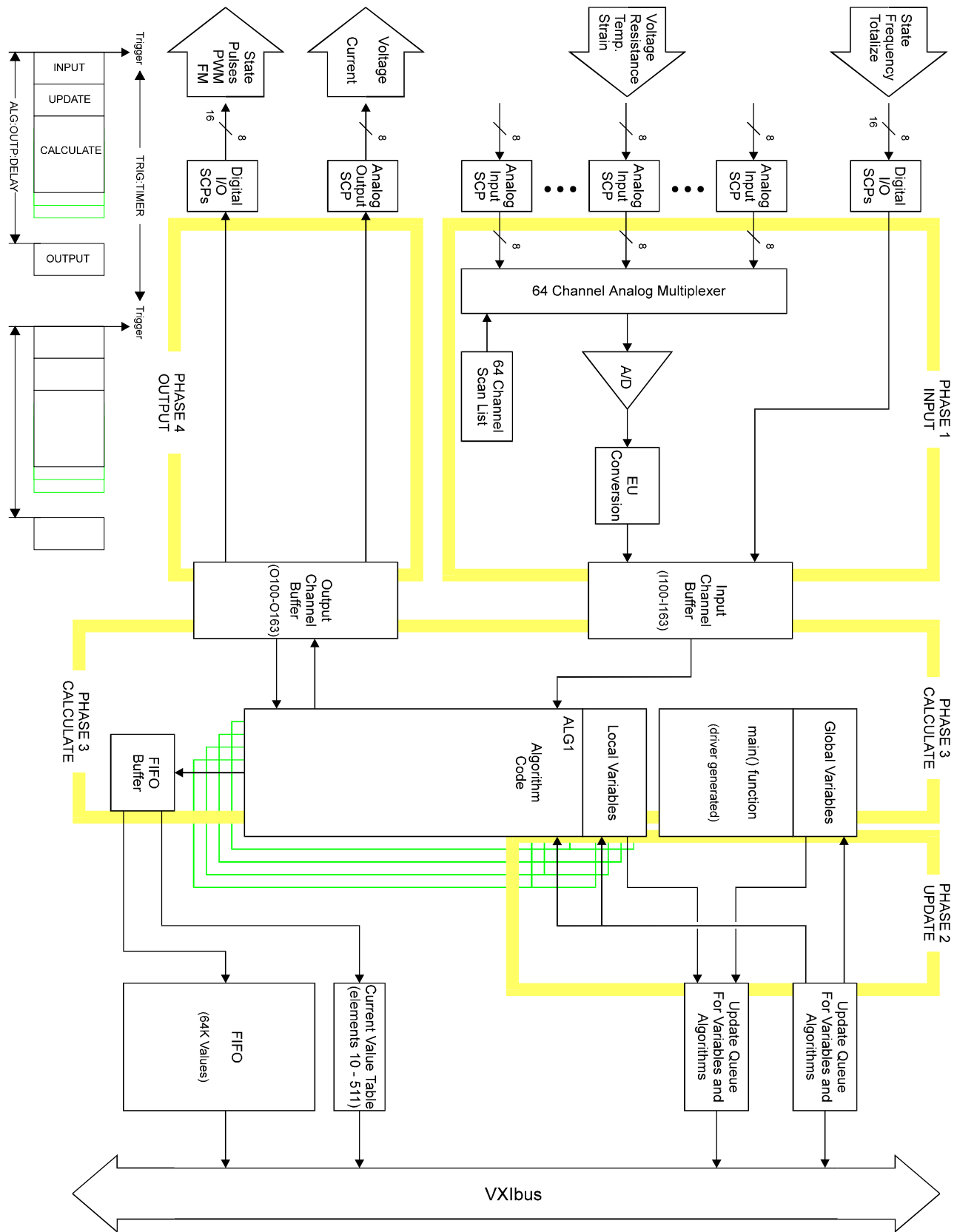
4-2 Algorithm Operating Sequence Diagram
