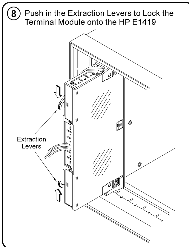
Figure 2-13 Wiring and Connecting the E1419 Terminal Module (Cont.)
