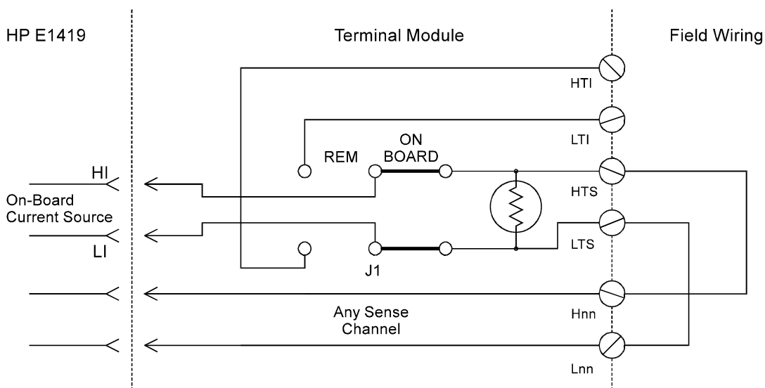
Figure 2-7 On-Board Thermistor Connections
