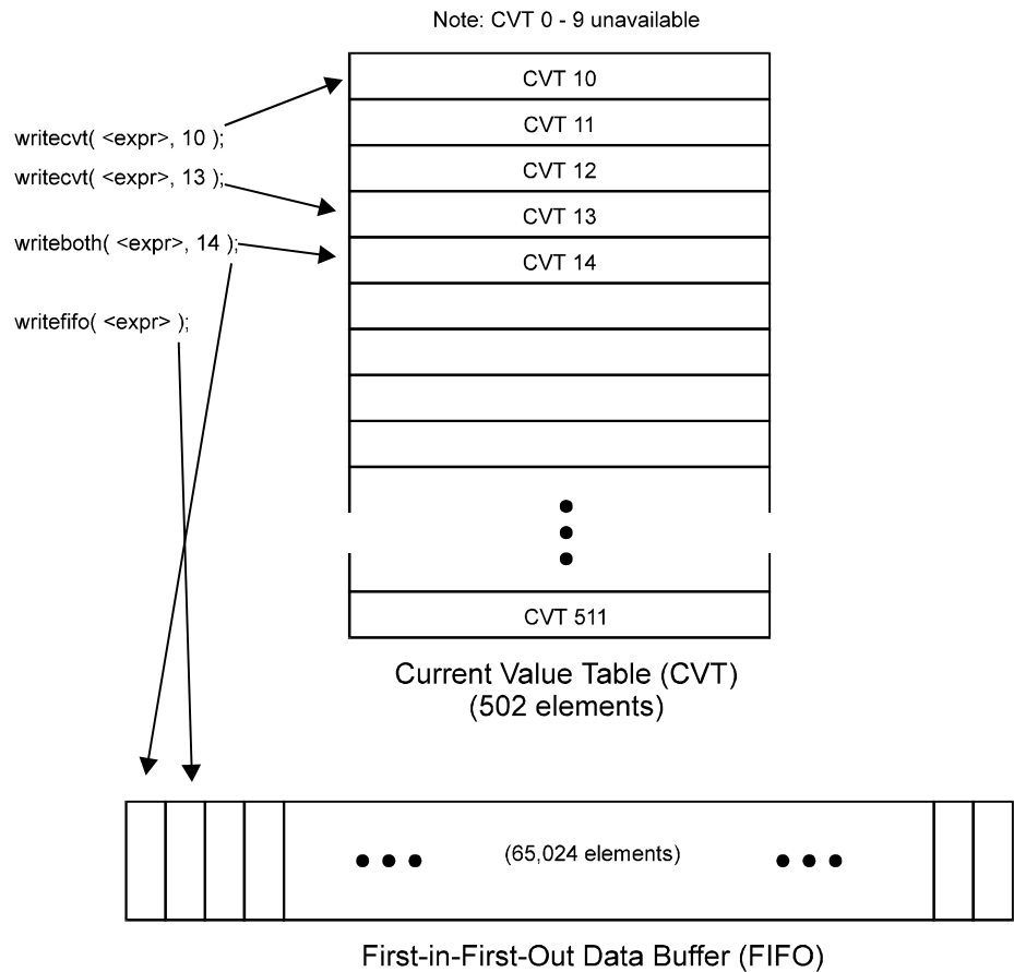
Figure 3-9 Writing Algorithm Data to FIFO and CVT
