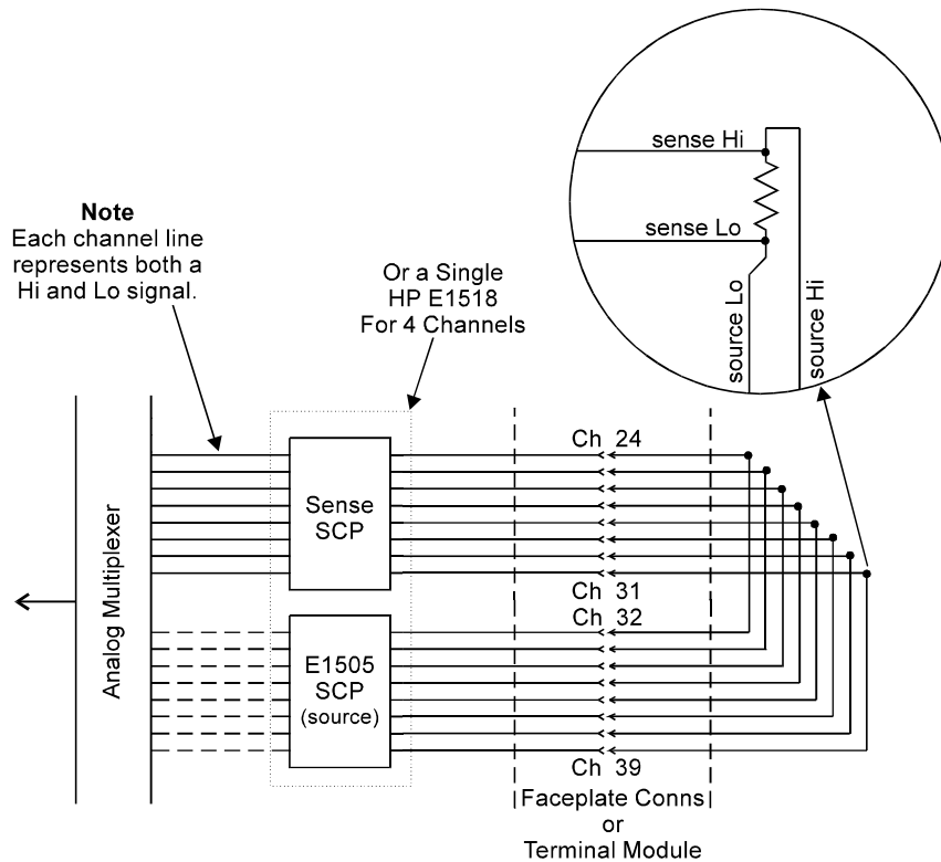
Figure 2-2 Pairing Source and Sense SCP Channels
