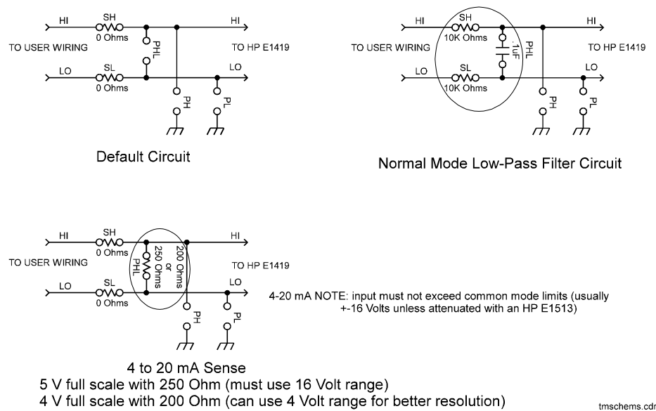
Figure 2-17 Series & Parallel Component Examples
