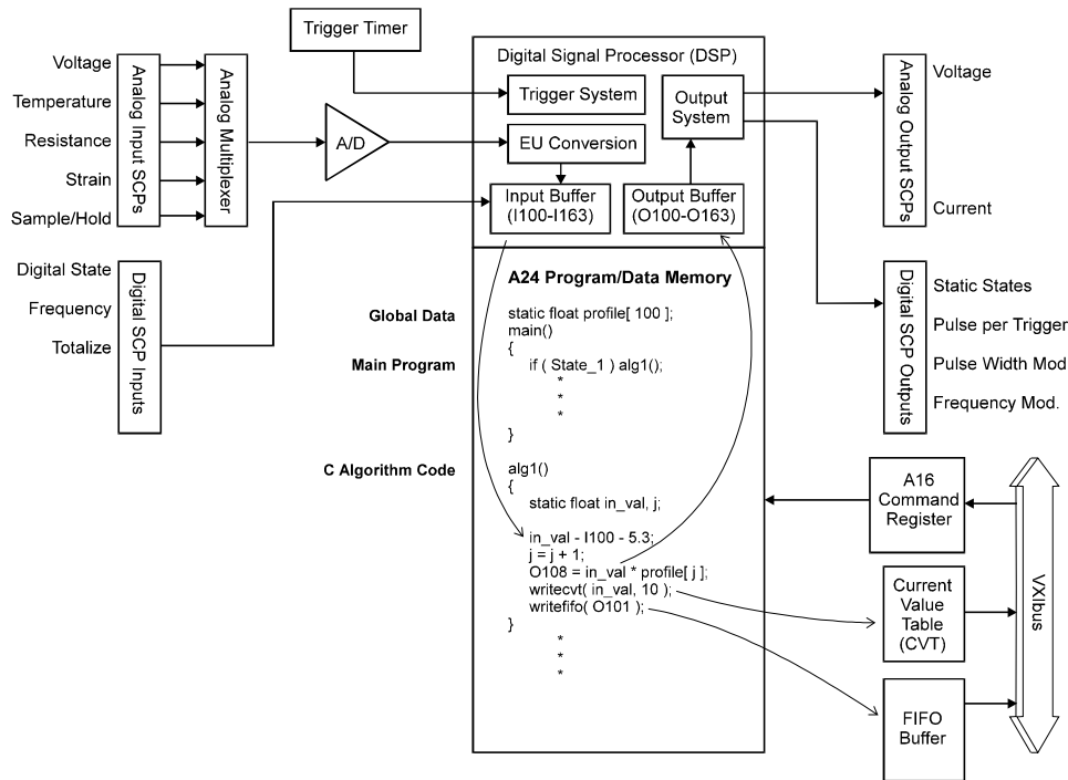
Figure 3-1 Simplified Functional Block Diagram
