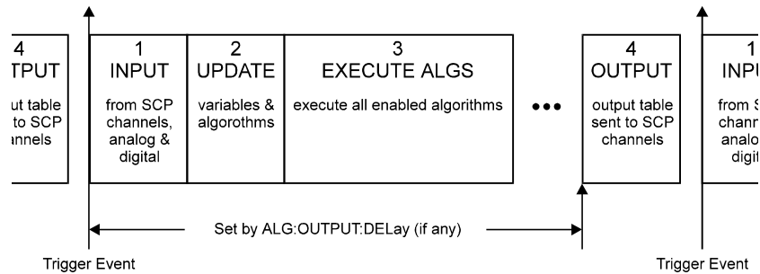
Figure 3-8 Sequence of Loop Operations
