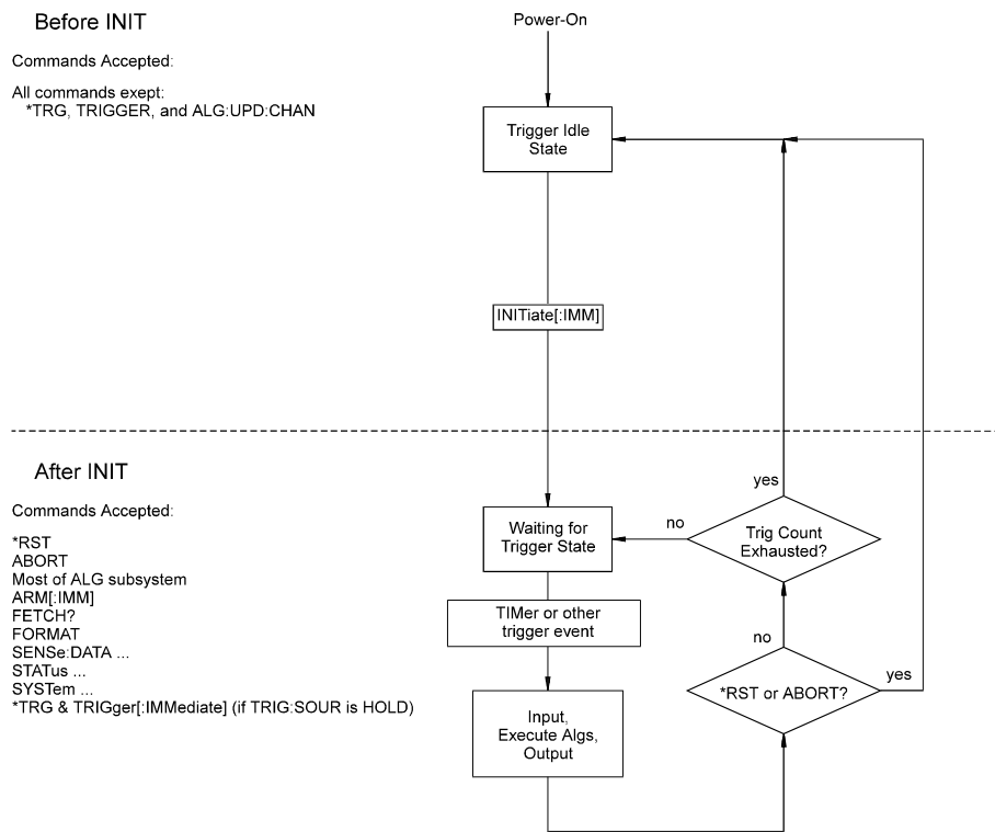
Figure 3-3 Module States
