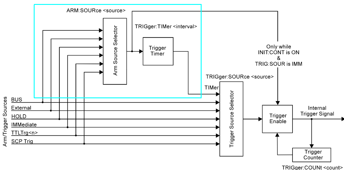
Figure 3-7 Logical Arm and Trigger Model
