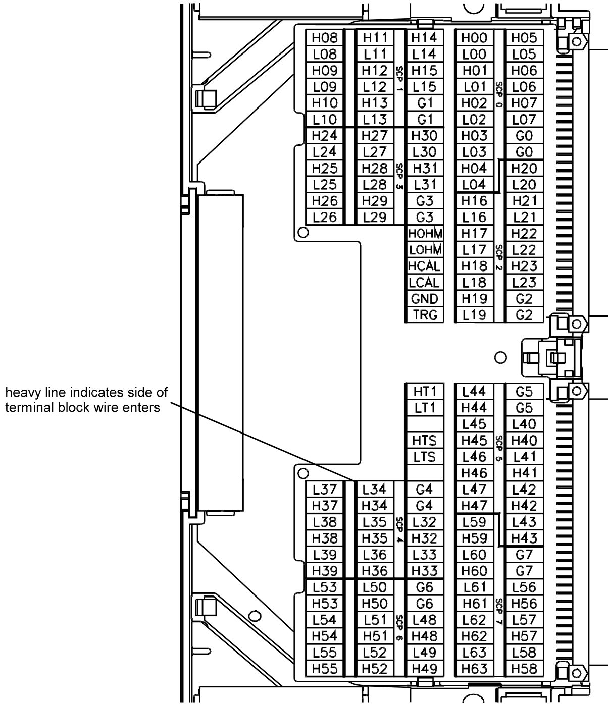
Figure 2-18 HP E1419A Option 11 Terminal Module Map
