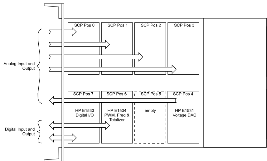
Figure D-1 Separating Analog and Digital Signals
