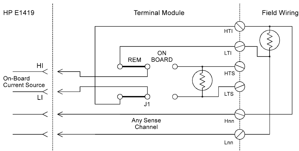
Figure 2-6 Remote Thermistor or RTD Connections
