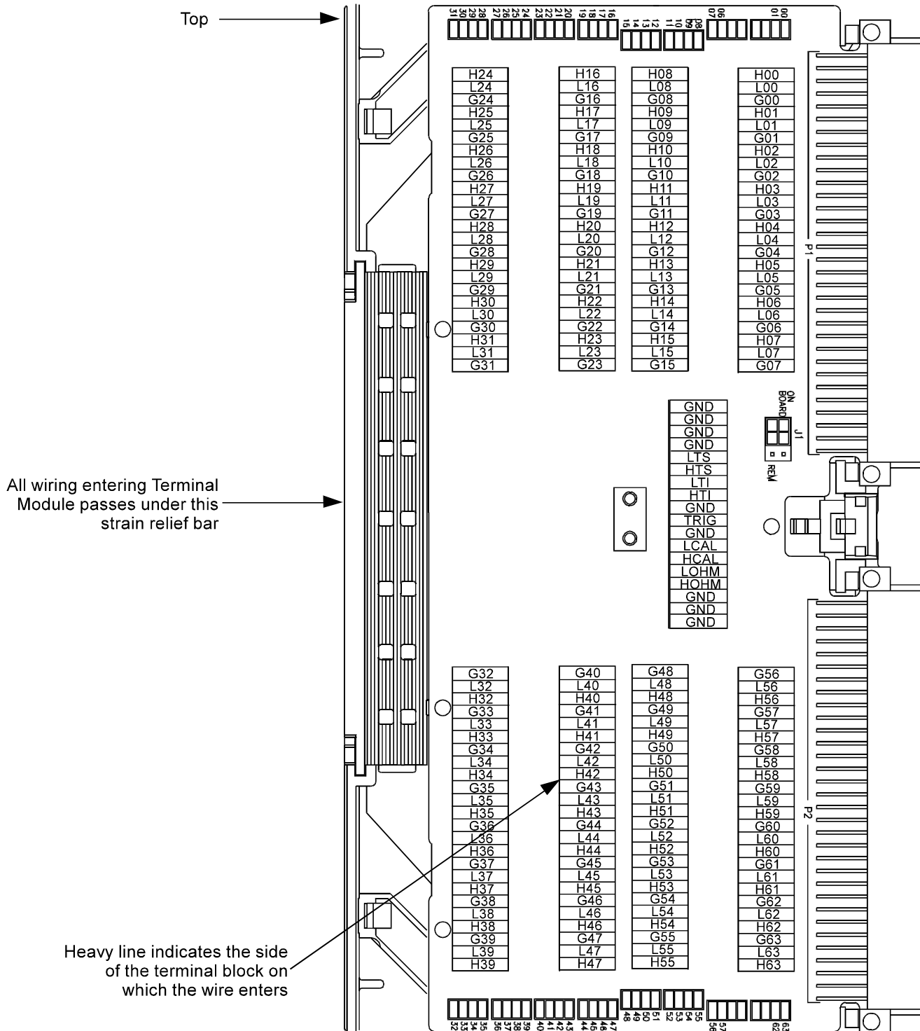
Figure 2-19 HP E1419A Option 12 Terminal Module Map
