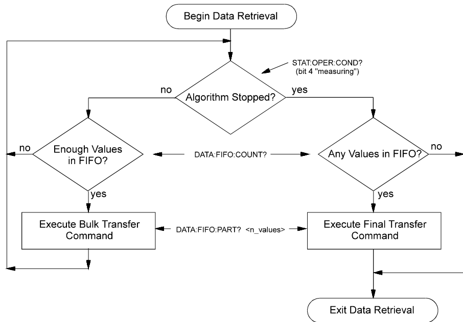
Figure 3-10 Controlling Reading Count
