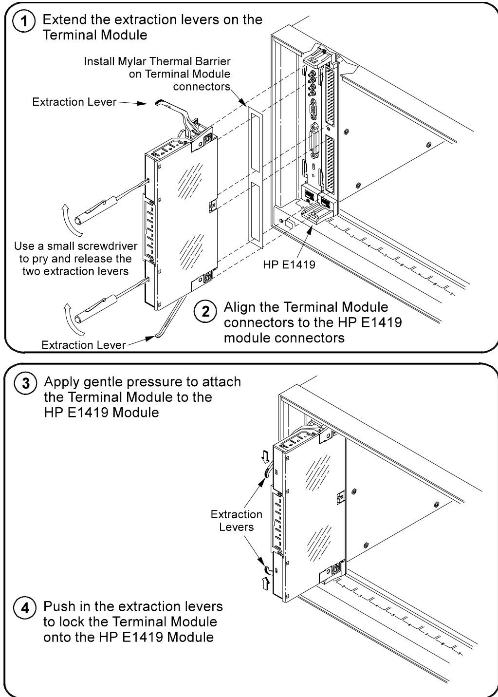
Figure 2-14 Attaching the HP E1419 Terminal Module
