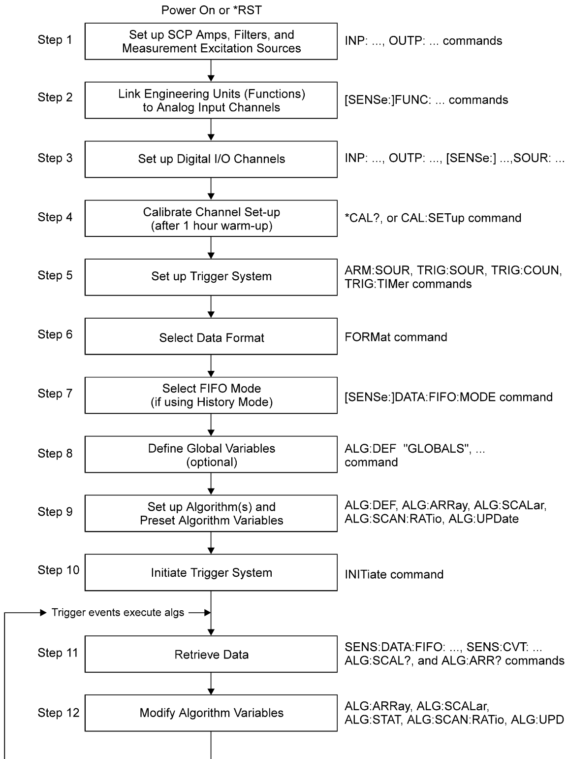
Figure 3-4 Programming Sequence
