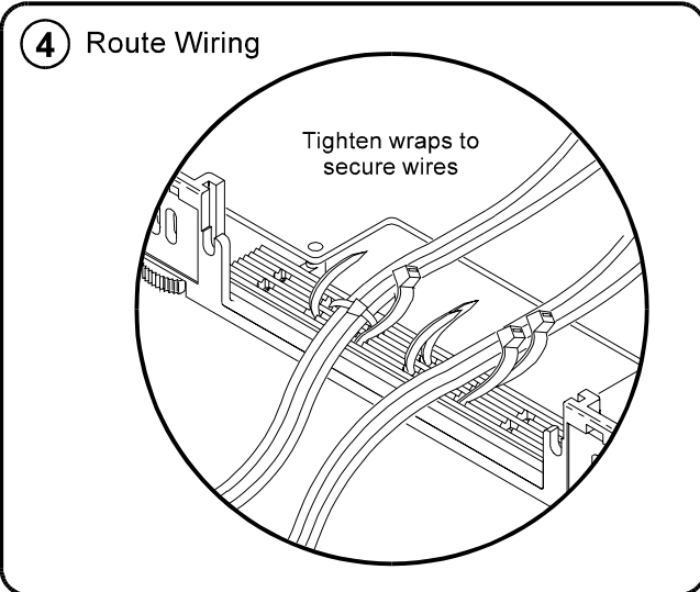
Figure 2-12 Wiring and Connecting the E1419 Terminal Module
