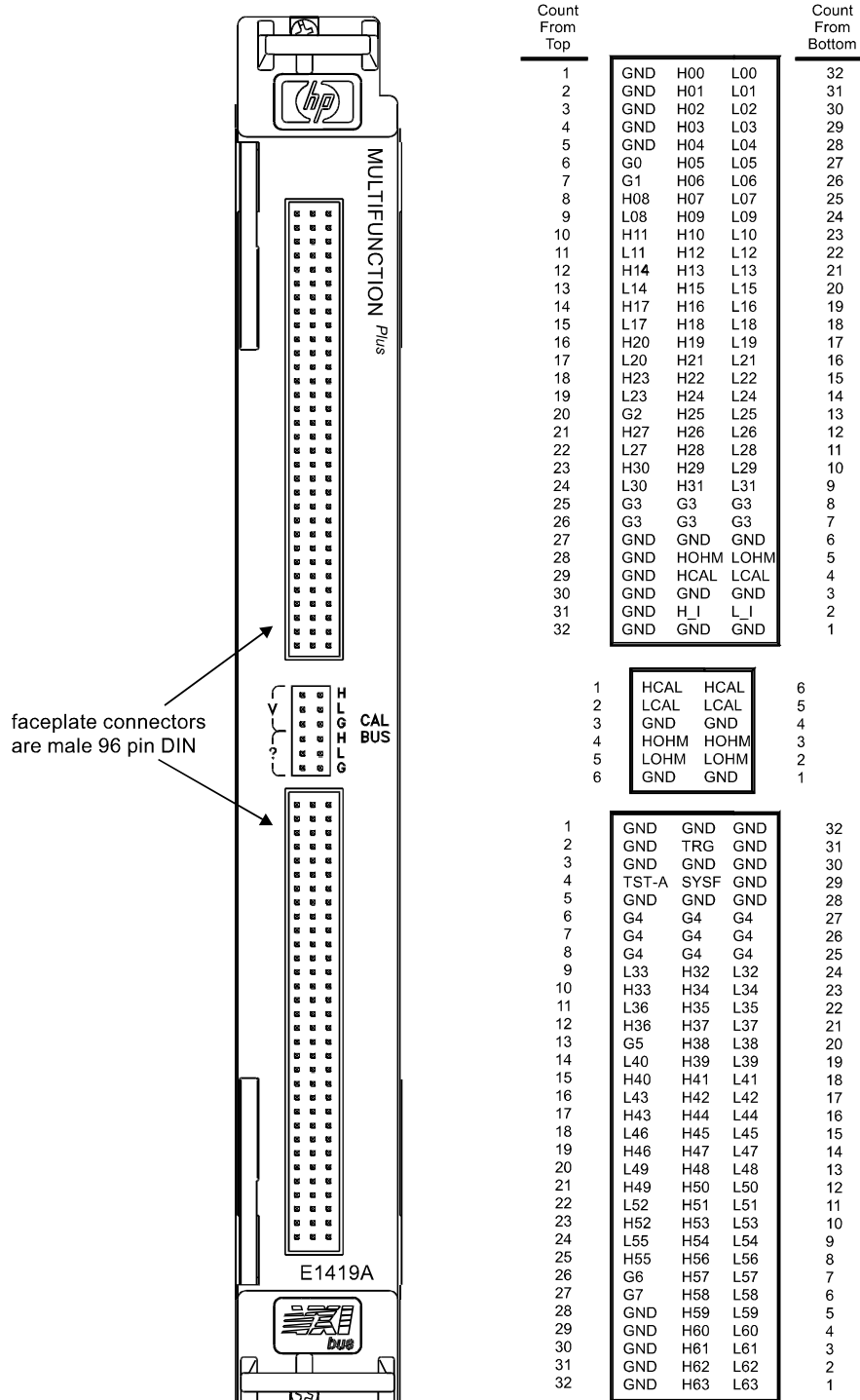
Figure 2-3 HP E1419A Faceplate Connector Pin Signals
