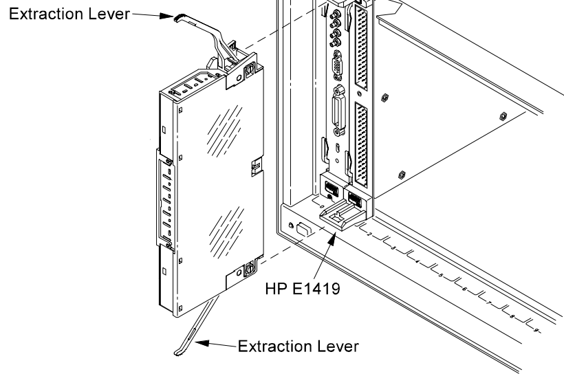
Figure 2-15 Removing the HP E149 Terminal Module
