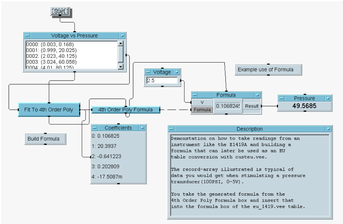
Figure 5-11 Curve Fitting and EU Generation
