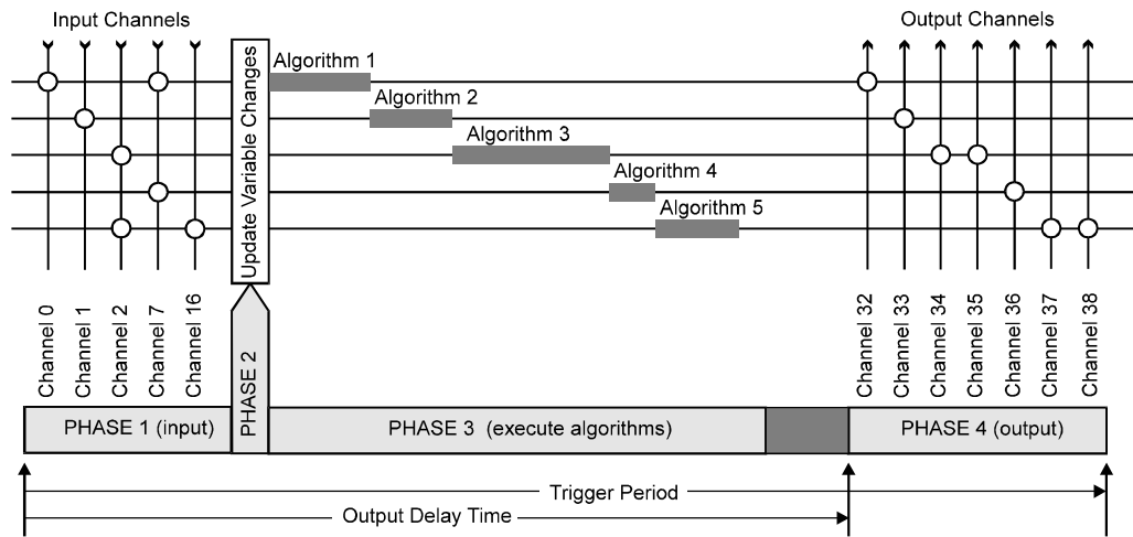
Figure 3-2 HP E1419A Cycle Phases
