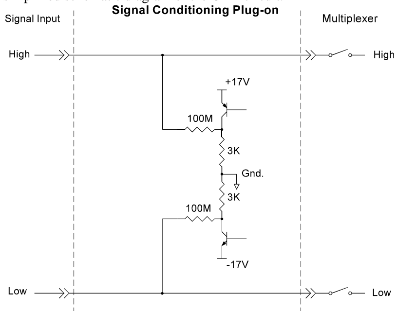
Figure 3-13 Simplified Open Transducer Detect Circuit
