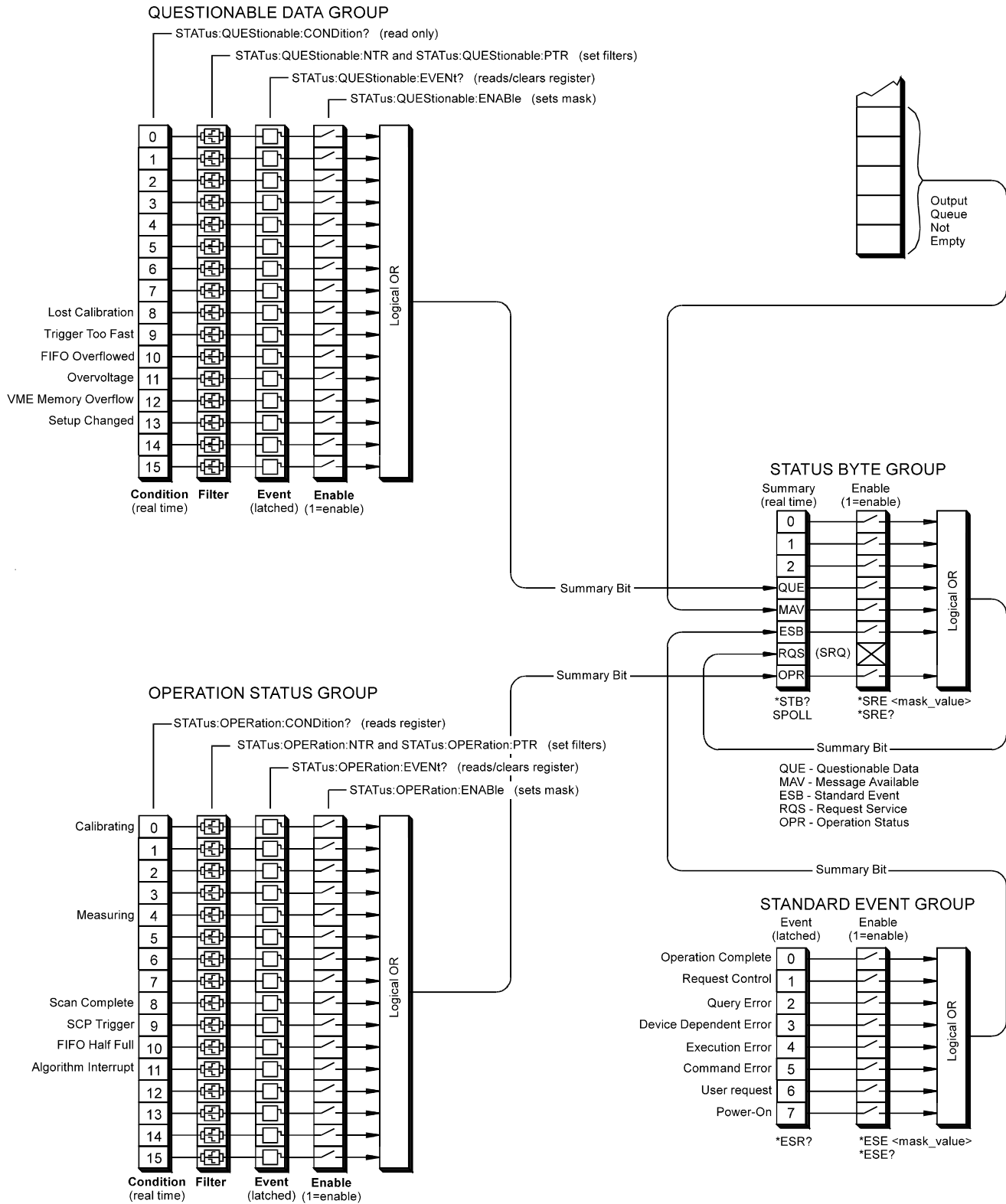
Figure 3-12 HP E1419 Status System
